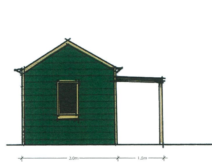
SIDE ELEVATION
